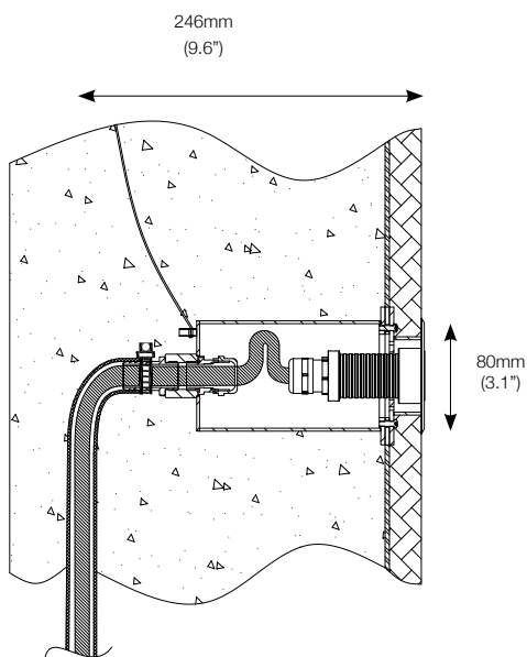
Trim (TM) AS402 - (TM)
