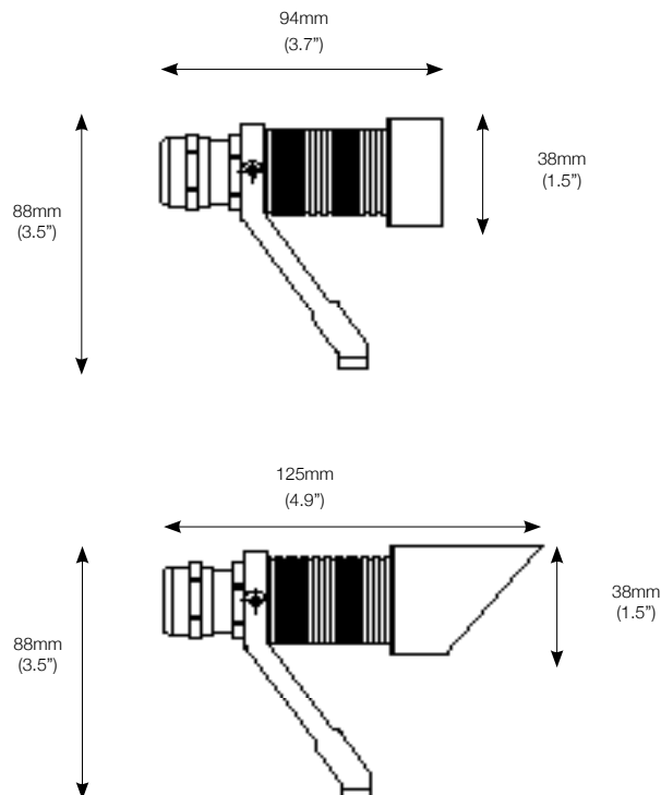
ASPS - Projector snoot
